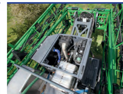
A powerful rear-mounted 230hp MTU engine optimises weight distribution and minimises cab noise and heat levels.
